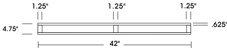
END VIEW
